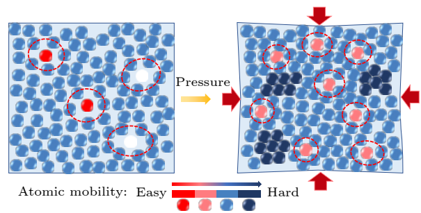
图 8 施加压力前后 \text{Fe}_{78}\text{Si}_9\text{B}_{13} 金属玻璃的原子结构示意图 Fig. 8. Schematic of atomic structure for \text{Fe}_{78}\text{Si}_9\text{B}_{13} metallic glass before and after applying pressure.
