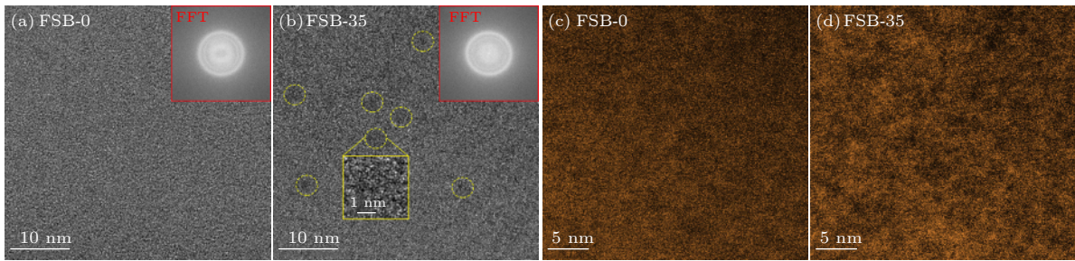
图 6 \text{Fe}_{78}\text{Si}_9\text{B}_{13} 金属玻璃未变形 (a) 和变形 (b) 的 HRTEM 图像, 插图是相对应的 FFT 模式, 黄色的圆圈标出了低亮度的区域; \text{Fe}_{78}\text{Si}_9\text{B}_{13} 金属玻璃未变形 (c) 和变形 (d) 的环形暗场扫描 TEM (ADF-STEM) 图像 Fig. 6. HRTEM images of the undeformed (a) and deformed (b) \text{Fe}_{78}\text{Si}_9\text{B}_{13} metallic glasses. The insets are the corresponding FFT patterns, and the yellow circles mark the regions with low brightness. Annular dark-field scanning TEM (ADF-STEM) images of the undeformed (c) and deformed (d) \text{Fe}_{78}\text{Si}_9\text{B}_{13} metallic glasses.
