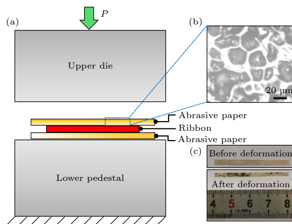
图 1 (a) \text{Fe}_{78}\text{Si}_9\text{B}_{13} 非晶带材施加载荷的示意图; (b) 砂纸的金相显微图像; (c) 样品变形前后的光学图片 Fig. 1. (a) Schematic diagram for the stress applying procedure of the \text{Fe}_{78}\text{Si}_9\text{B}_{13} amorphous ribbon; (b) metallographic microscope images of the abrasive paper; (c) optical picture of samples before and after deformation.
