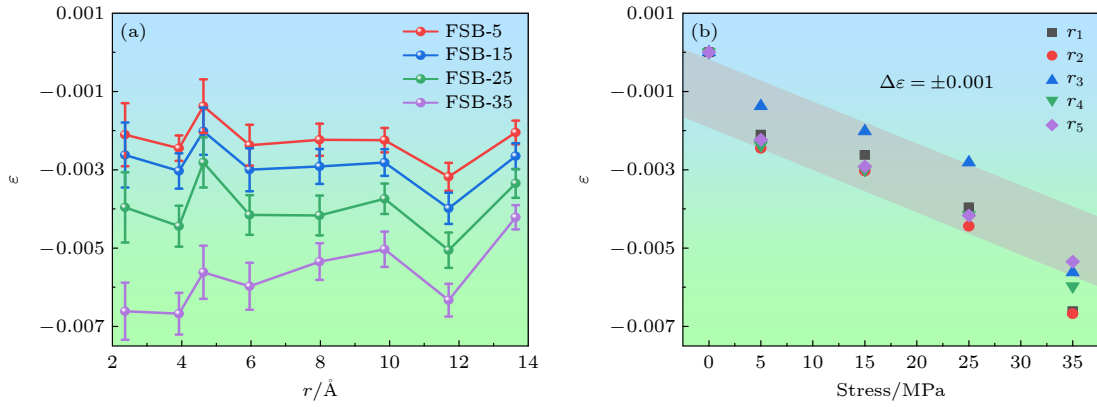
图 5 (a) 由 G(r) 曲线峰位置的相对位移确定的不同压力下 \text{Fe}_{78}\text{Si}_9\text{B}_{13} 金属玻璃的体积应变 \varepsilon ; (b) \varepsilon 随压力的变化 Fig. 5. (a) Volume strain \varepsilon of \text{Fe}_{78}\text{Si}_9\text{B}_{13} metallic glasses at various pressures determined from the relative displacement of the peak position of the G(r) ; (b) the variation of \varepsilon with pressure.
