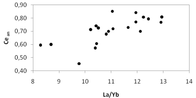
Fig. 15. Ce_{an} versus La/Yb diagram along the phosphatic section of Oum El Khecheb showing a positive correlation between Ce_{an} values and the REE fractionation ( La/Yb ).
