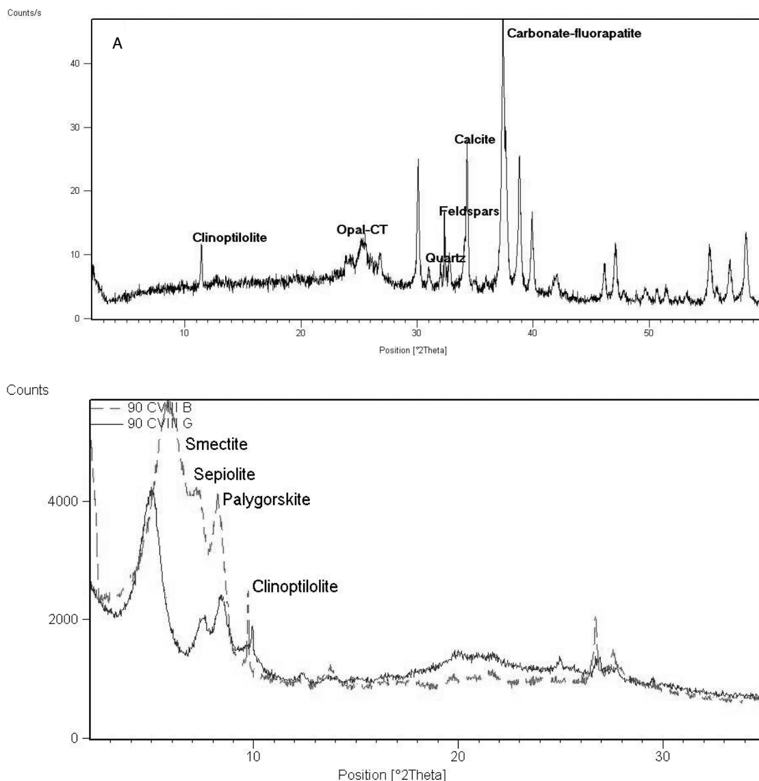
Fig. 4. A: XRD diagrams of powder sample 90 CVIII. B: XRD clays diagrams of sample 90 CVIII (90 CVIII B: untreated and 90 CVIII G: glycolated).
