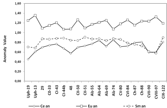
Fig. 17. Ce, Eu and Sm anomalies distribution along the Oum El Khecheb phosphorites profile.
