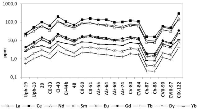
Fig. 10. Rare earth elements distribution (La, Ce, Nd, Sm, Eu, Gd, Tb, Dy and Yb) along the phosphatic section of Oum El Khecheb (GMB; Tunisia). (Uph: Upper Phosphate; Alz: Alternation Zone and Ch: cherts).
