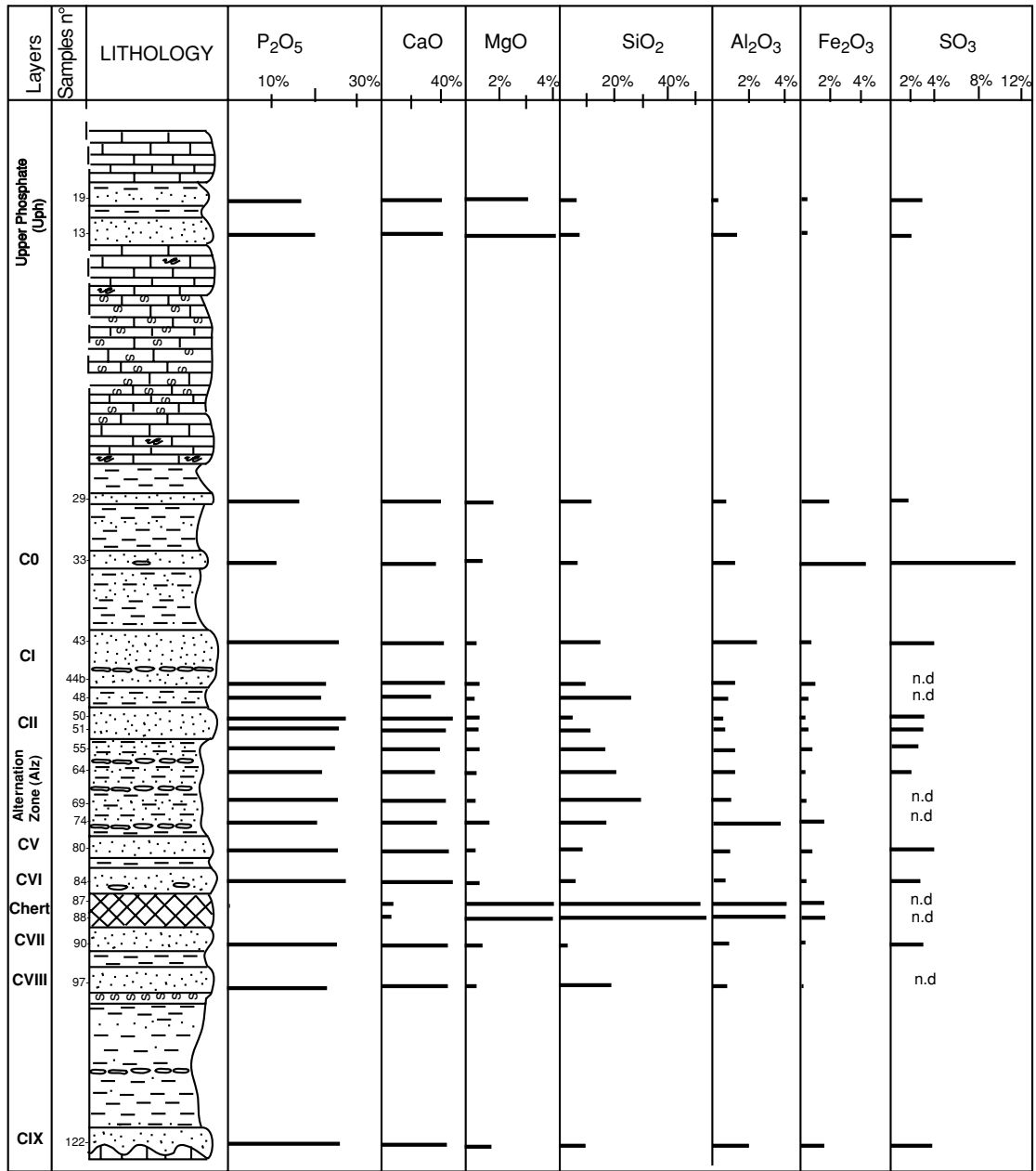
Fig. 7. Variation of the chemical composition in the main layers of phosphorites and chert of Oum El Khecheb profile.
