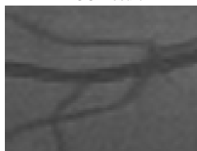
SRCNN result
