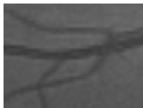
Proposed method
