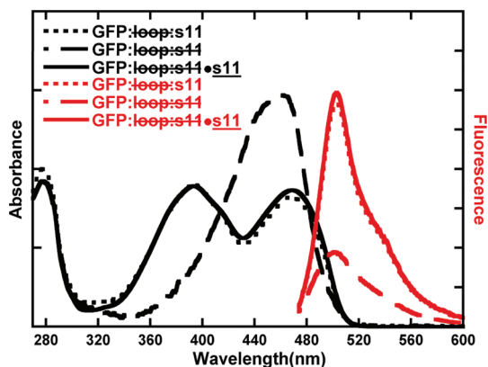
Figure 3. Absorbance and fluorescence spectra of elements in method described in Figure 2A for the removal and replacement of strand 11. GFP:loop:s11, GFP:loop:sH, and GFP:loop:sH*s11 spectra are shown by dotted, dashed, and solid lines, respectively. The spectra of GFP:loop:sH*s11 and GFP with s11 covalently attached are nearly identical 1 (data not shown). The absorbance spectrum of GFP:loop:sH has a single band in the visible region unlike the parent protein with s11 covalently or noncovalently attached. All spectra are normalized by concentration so that the relative intensities of the absorbance spectra reflect differences in extinction coefficients and the emission spectra relative intensities reflect the difference in extinction coefficient and quantum yield upon excitation at 468 nm.
