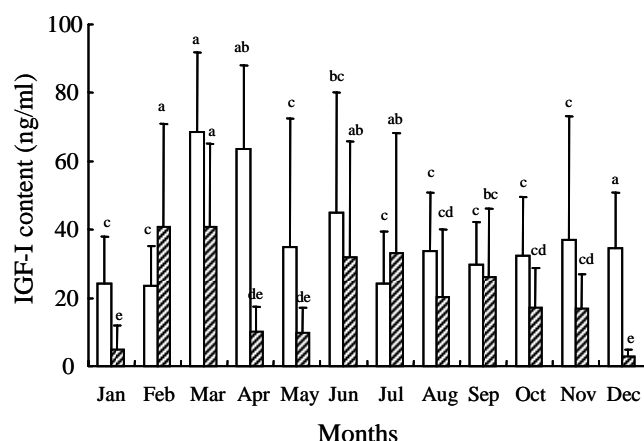
Figure 1. IGF-I concentration throughout an year period in whey at two farms. Open bars located in each month represent content of milk IGF-I in farm A ( n = 320 ), and hatched bars represent in Farm B ( n = 325 ). Different letter superscripts indicate differences at p < 0.05 .
