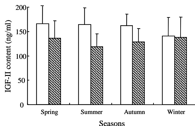
Figure 2. IGF-II concentration throughout seasons in whey at two farms. Open bars represent content of milk IGF-II in Farm A ( n = 47 ), and hatched bars represent in Farm B ( n = 57 ). Different letter superscripts indicate differences at p < 0.05 .
