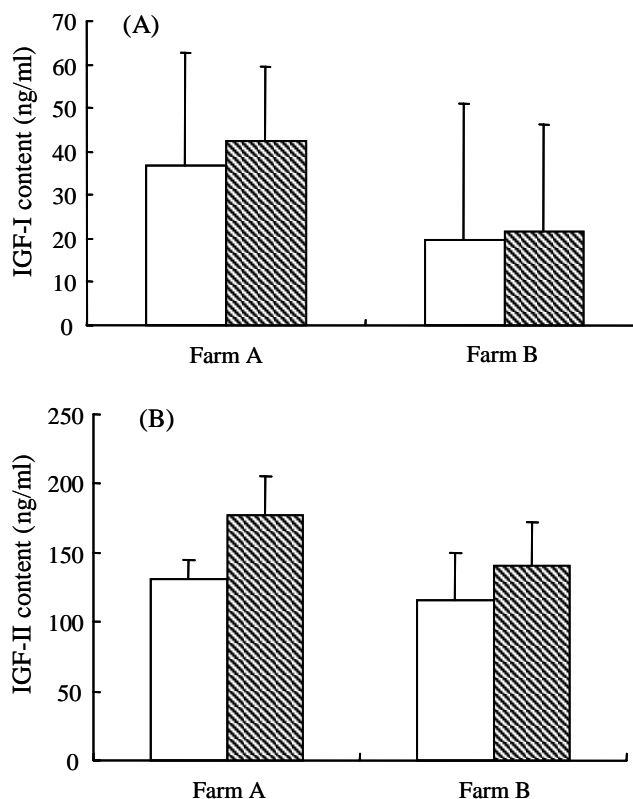
Figure 4. Mean IGF-I (A) and IGF-II (B) concentrations in primiparous and multiparous whey. Open bars represent primiparous IGF-I content, and hatched bars represent multiparous, shown as the mean±SEM.
