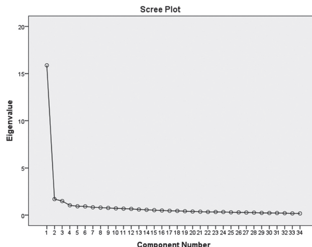
Fig. 1. Scree plot showing eigenvalues of the components.
