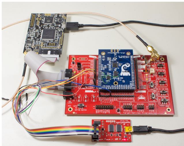
Figure 7. Power analysis on the AT-Mega2564RFR2 from a Philips Hue bulb was done using a ChipWhisperer-Lite (top left), connected to a custom PCB with the AT-Mega2564RFR2 mounted (middle blue PCB), using a Bus Pirate (bottom small PCB) to reprogram a SPI flash chip with various byte sequences.
