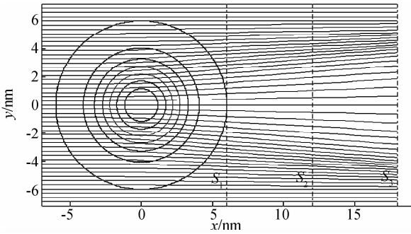
图 2 编码光束经过等离子体在空间传输 Fig. 2 The transportation of coded probing rays
