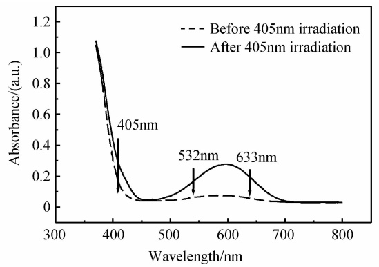
图 2 聚合物薄膜在激励光照前后的吸收光谱 Fig. 2 Absorption spectrum of polymer film before and after irradiation
