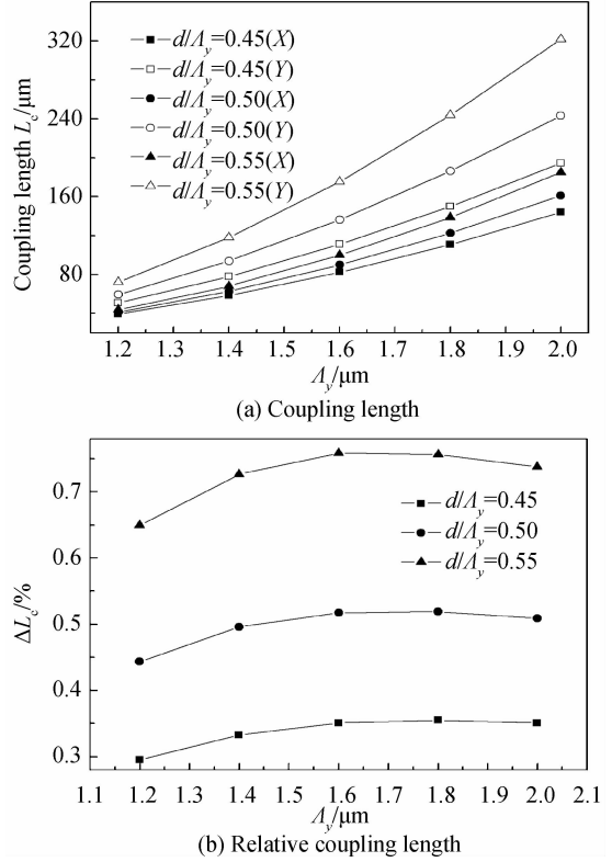
图 3 \Lambda_x/\Lambda_y = 0.6, b = d, \eta = 1 时, d/\Lambda_y 从 0.45 变化到 0.55, 耦合长度和相对耦合长度随 \Lambda_y 的变化 Fig. 3 Coupling length and relative coupling length as a function of hole-pitch \Lambda_y under different d/\Lambda_y
