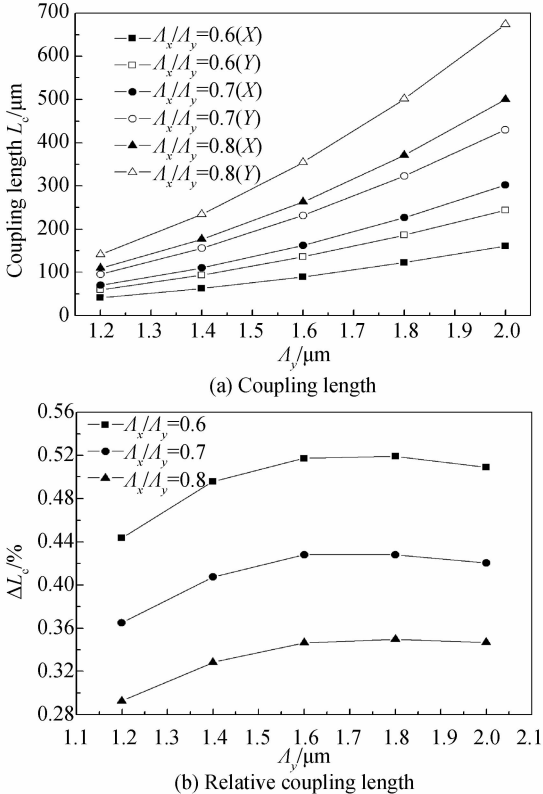
图 2 d/\Lambda_y = 0.5, b = d, \eta = 1 时, \Lambda_x/\Lambda_y 从 0.6 变化到 0.8, 耦合长度和相对耦合长度随 \Lambda_y 的变化 Fig. 2 Coupling length and relative coupling length as a function of hole-pitch \Lambda_y under different \Lambda_x/\Lambda_y
