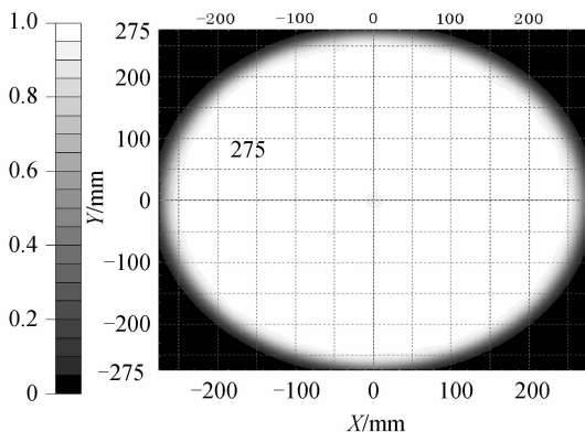
(b) Illumination distribution of a/b=4/9
