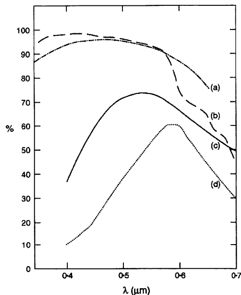
Figure 6. The percent transmittance in the visible band through one meter of water for various water types: (a) Clear Mediterranean, (b) Crater Lake, (c) coastal: medium transparency, (d) coastal: low transparency (Kraus and Businger, 1994). Copyright Oxford University Press.
