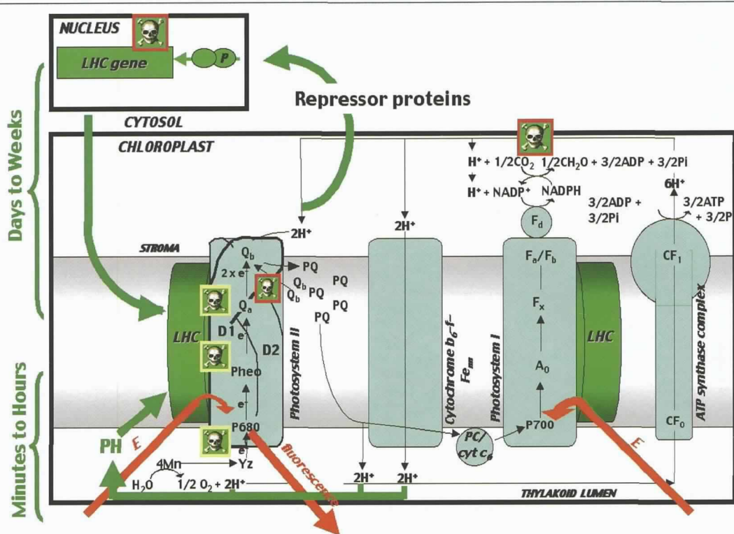
Figure 16. The chemical reactions that convert radiant energy into chemical energy. A complete description of the light and dark reactions can be found in Falkowski and Raven (1998). The red arrows delineate the incoming light absorbed by the light harvesting complexes (LHCs) and the fluorescently emitted light by the phytoplankton. The absorbed light results in a stable charge separation and the electron is passed through a series of molecules, illustrated by the black arrows, with the net result being the formation of oxygen and organic carbon ( \text{CH}_2\text{O} ). The amount of \text{CH}_2\text{O} produced is dependent on the amount of light absorbed and the efficiency with which the absorbed radiation is utilized. The amount of light that is absorbed for photosynthesis is variable as the photosynthetically-active optical cross-section is adjusted by several different photo-acclimation processes (the green arrows). Over short time scales (minutes and hours), pigments can be inter-converted between photosynthetically-active and nonphotosynthetically-active pigments. Over longer time scales (days to weeks) pigment concentrations can be increased via nuclear-driven pigment synthesis. Both of these acclimation processes are coupled to the photosynthetically-induced pH gradient present across the thylakoid membrane (Demmig-Adams, 1990; Escoubas et al., 1995). The efficiency with which the absorbed light is utilized is impacted by the nutrient status of the cells, which provides the material to build the biochemical scaffolding required for photosynthesis. Secondly, if visible and ultraviolet light radiation levels are excessive, the photosynthetic efficiency can be decreased from light-induced damage within the cell. The hypothesized target sites for visible (yellow outlined skulls) and ultraviolet (red outlined skulls) are delineated.
