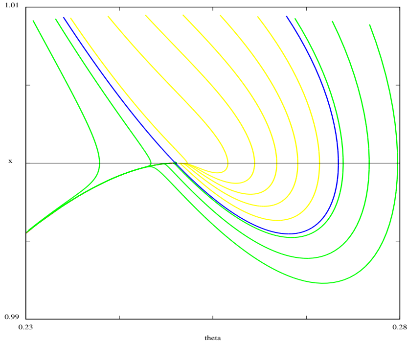
Figure 4.3. The flow of \Psi_h near a saddle-node. Trajectories in the strong stable manifold are drawn in blue, trajectories in the interior of the stable manifold are drawn in yellow, and trajectories in the hyperbolic region are drawn in green.
