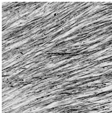
Figure 11. Image with Oriented Linear Features.
