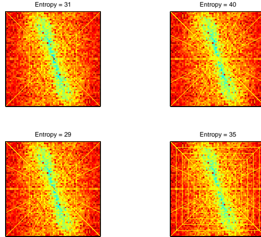
Figure 13. The two-dimensional Fourier transform overlaid with tilings defining 4 different ridgelet packet bases; the labels give the number of coefficients above threshold. Apparently, a decomposition splitting only on directions gives a larger number of coefficients exceeding threshold; while a decomposition splitting into more angular bins at higher frequencies gives fewer coefficients exceeding threshold..
