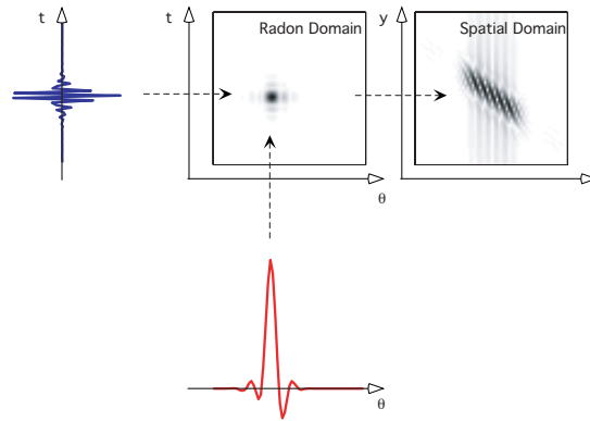
Figure 3. Construction of a Ridgelet Packet. A wavelet packet in the ridge direction and father wavelet Symmlet 8 in the angular direction are combined by tensor product, creating a waveform in the normalized Radon domain; this is backprojected into the spatial domain, creating an oriented waveform there.
