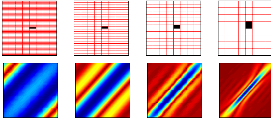
Figure 9. Basis Functions Derived from Tiles of Varying Heights.
