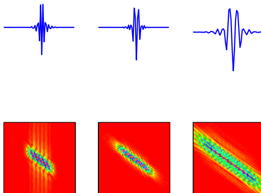
Figure 10. Basis functions derived from Radon-domain approach. Backprojections of Wavelet Packets at Different Widths in the ridge direction give different spatial waveforms.
