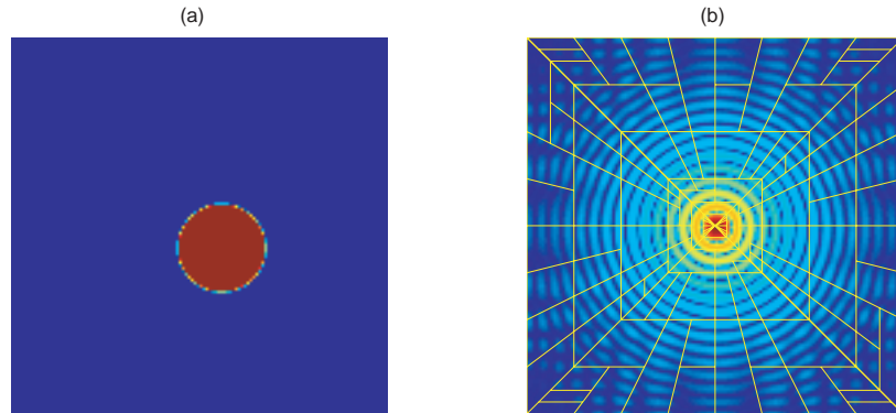
Figure 5. Disc-shaped object and Adapted Tiling. (a) Disc-shaped object. (b) Adaptive Tiling of the Fourier Plane, overlaid on the Fourier Transform of the disc. It is interesting to note that owing to the Cartesian structure of the data, the Fourier Transform of the disc does not have radial symmetry near the corners. This may explain the ‘unexpected’ high-frequency splits..
