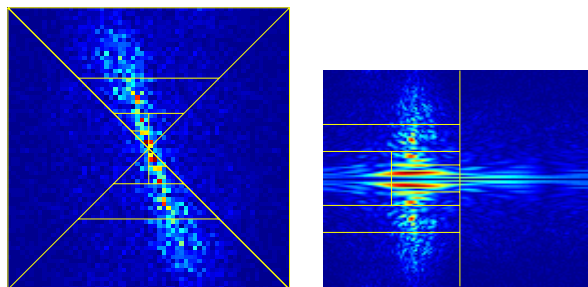
Figure 14. Left panel: Best rectangular partition overlaid on pseudopolar Fourier Plane. Right panel: Corresponding tiling of Cartesian Fourier Plane.
