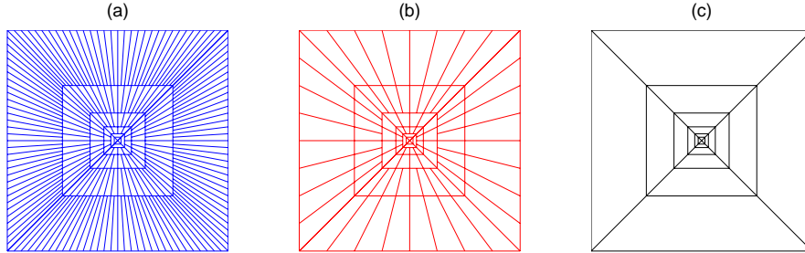
Figure 4. Three Tilings of the Digital Frequency Domain: (a) Digital Ridgelet; (b) Digital FIO; (c) Wavelet-like.
