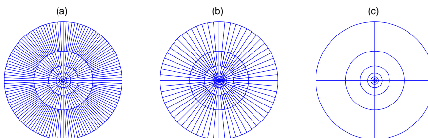
Figure 1. Three Tilings of the Frequency Domain: (a) Ridgelet tiling; (b) FIO tiling; (c) Wavelet tiling.
