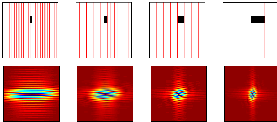
Figure 8. Basis Functions Derived from Tiles of Different Widths.
