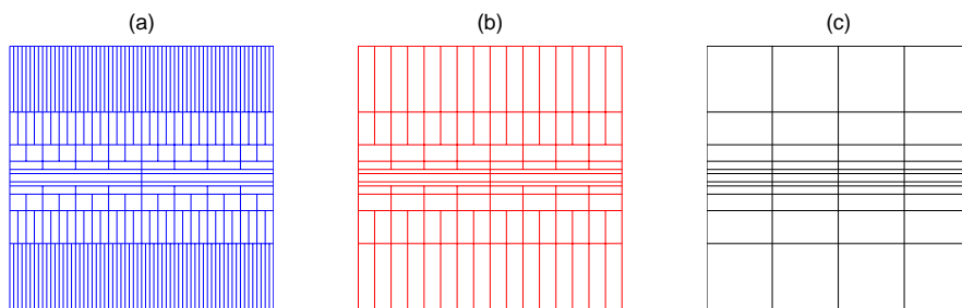
Figure 6. Tilings of Figure 1 Translated into Polar Form.
