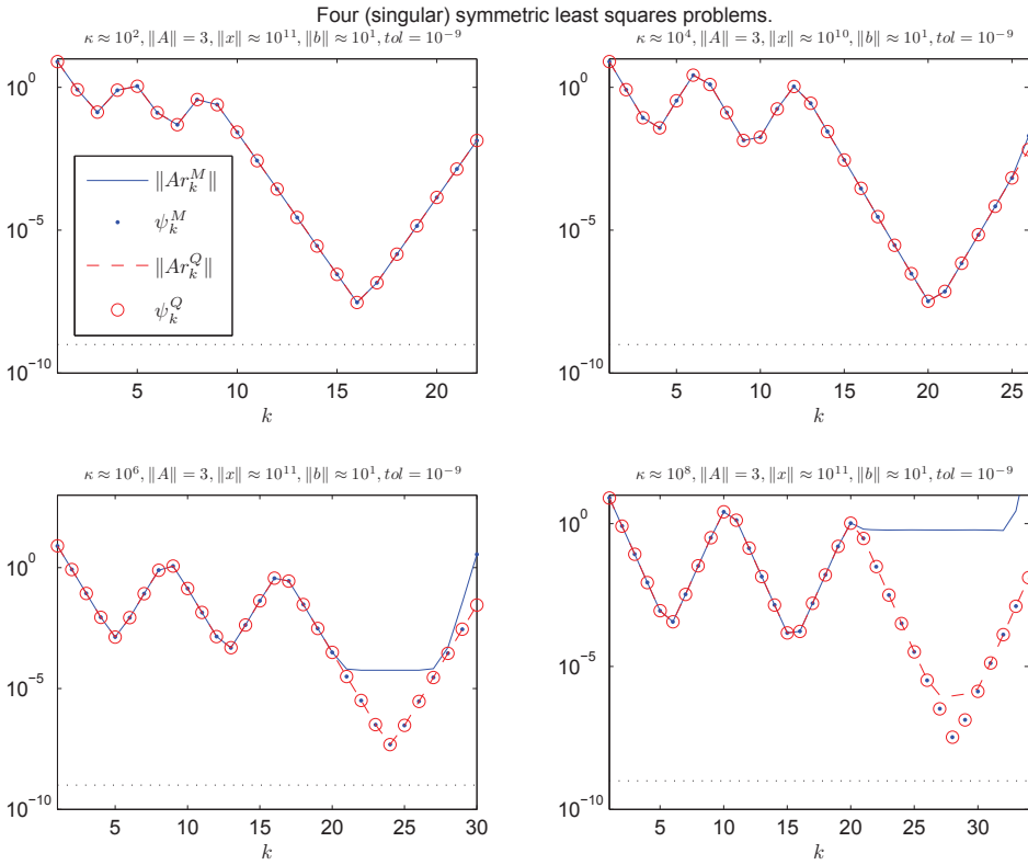
FIG. 8.3. Solving Ax = b with semidefinite A similar to an example of Sleijpen, Van der Vorst, and Modersitzki [47]. A = Q \text{diag}([0_5, \eta, 2\eta, 2 : \frac{1}{789} : 3])Q of dimension n = 797 with \|A\| = 3 , where Q = I - (2/n)ee^T is a Householder matrix generated by e = [1, \dots, 1]^T . (We are not plotting the NRBE quantities because \|A\|\|r_k\| \approx 6 throughout the iterations in this example.)
