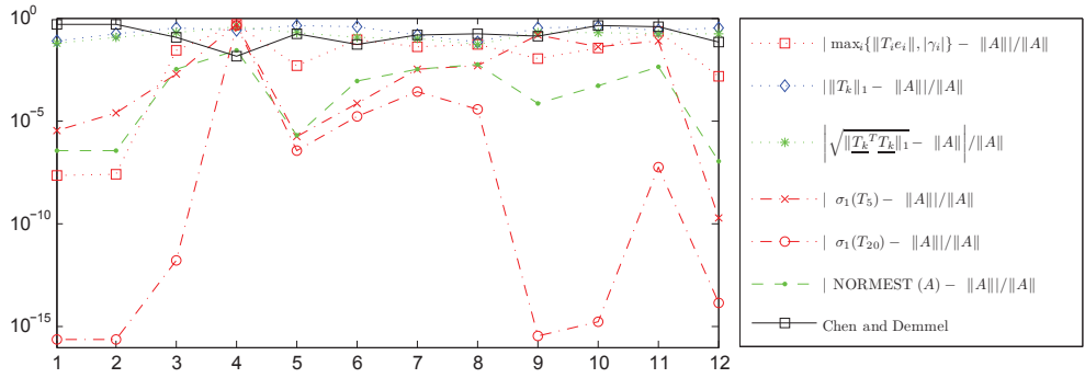
FIG. 6.1. Relative errors in different estimates of \|A\| . This figure can be reproduced by testminresQLPNormA3 .
