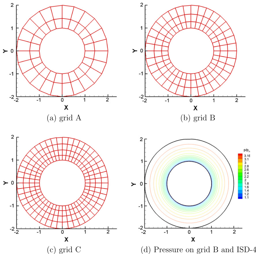
Fig. 2. Meshes for incompressible Taylor-Couette flow.
