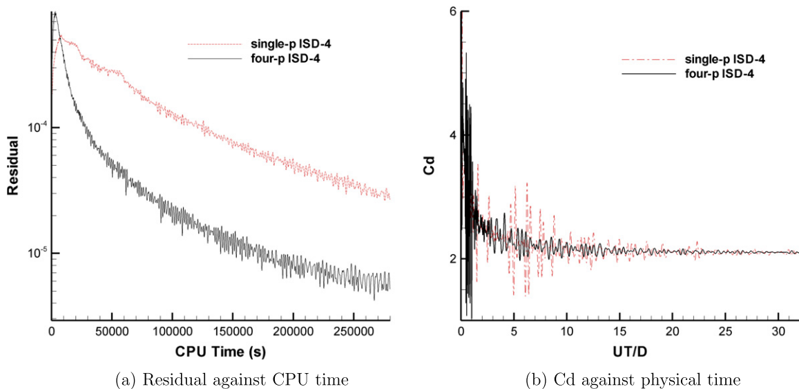
Fig. 9. Solution convergence rates for the fourth-order ISD method on a single- p grid and a four-level p -multigrid.
