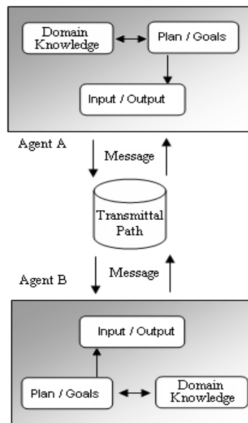
Figure 1. Distributed Information Agents communicating with each other
