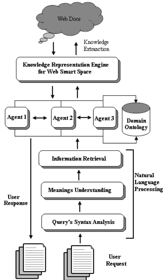
Figure 2. A Web Smart Space Framework for Information Mining
