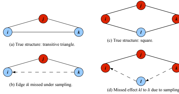
FIGURE 2. Red nodes are sampled. (a) and (c) show examples of true network structures. (b) shows the star subgraph from (a) when j is sampled. The effect of k on i is missed. (d) shows the induced subgraph from (c) when i , j , and k are sampled. The effect of k on i through l is missed.
