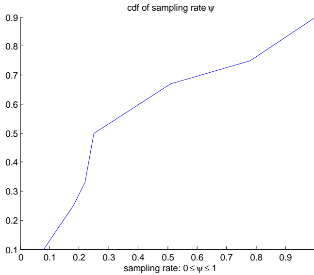
FIGURE 3. A CDF of the sampling rate in the literature. A detailed description of the literature survey is available from the author upon request.
