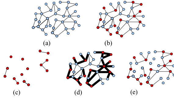
FIGURE 1. (a) G = (V, E) . (b) the sampled nodes, S , in red. (c) the induced subgraph, G^{l^S} = (S, E^{l^S}) . (d) G , highlighting the sampled nodes and the edges that are induced if each sampled node reports all of its links from the census, E^S . (e) the star subgraph, G^S .
