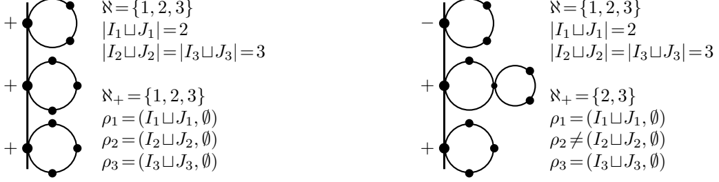
Figure 10: Typical elements of \widetilde{\mathcal{M}}_{0,\varrho}^0 and \widetilde{\mathcal{M}}_{0,\rho}^0
