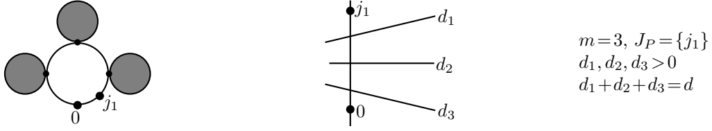
Figure 11: A typical element of \overline{\mathfrak{M}}_{0,\sigma}(\mathbb{P}^n, d)
