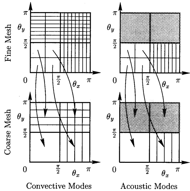
4b: Damping Schematic for Full Coarsened Multigrid.
