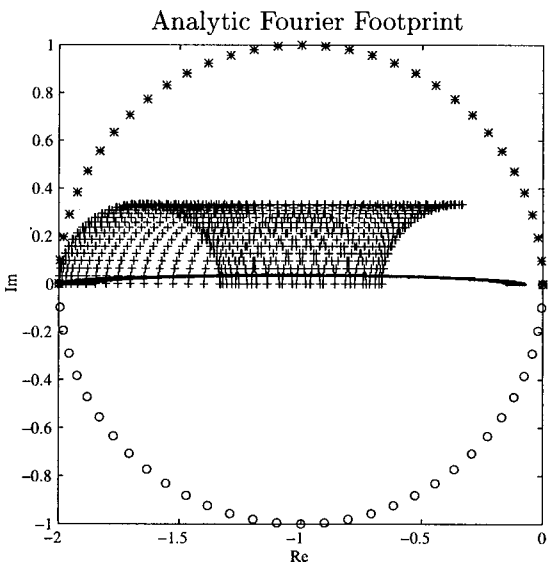
5a: Footprint for all modes except L_x L_y . Case NS1 with M = 0.04 .
