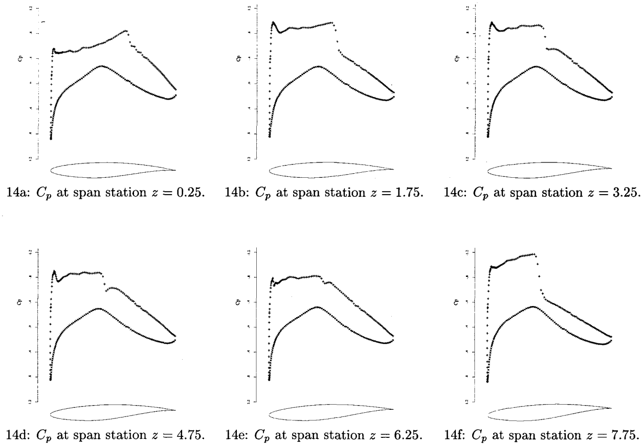
Figure 14: Spanwise pressure distributions for a wing with endplates. Geometry: RAE2822 Airfoil, Aspect Ratio = 8, Sweep = 30°, Twist = 3.5°. Flow conditions: M = 0.8 , \alpha = 4.0^\circ , Re = 6.5 \times 10^6 .
