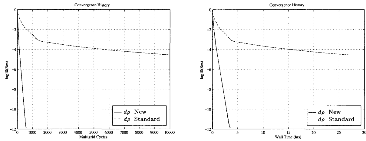
15a: Convergence comparison. 15b: Cost comparison. Figure 15: Fully-3D Wing: Comparison of the new and standard methods using the BL turbulence model.
