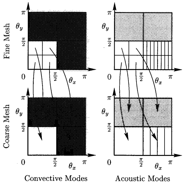
5b: Damping Schematic for Full Coarsened Multigrid.
