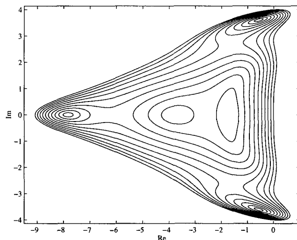
Figure 2: Stability region and contours defined by |\psi(z)| = 0.1, 0.2, \dots, 1.0 for a 5-stage Runge-Kutta time-stepping scheme.
