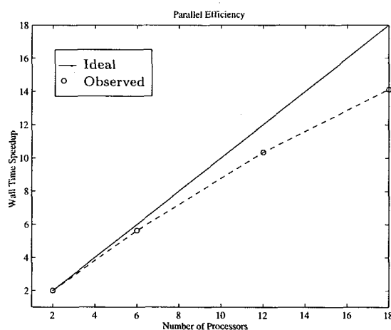
Figure 9: Parallel efficiency for a 288 \times 64 \times 16 mesh.
