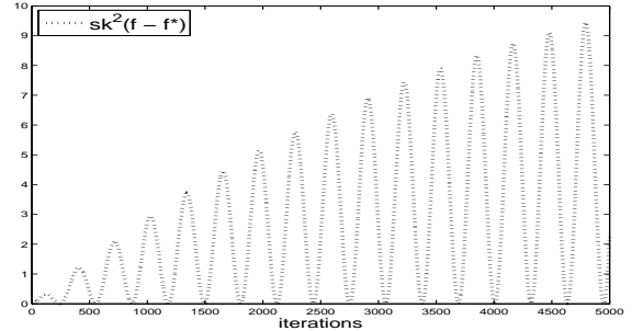
(b) Scaled errors sk^2(f(x_k) - f^*) .
