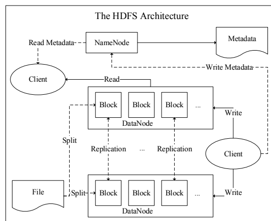
Figure 1. The HDFS Architecture
