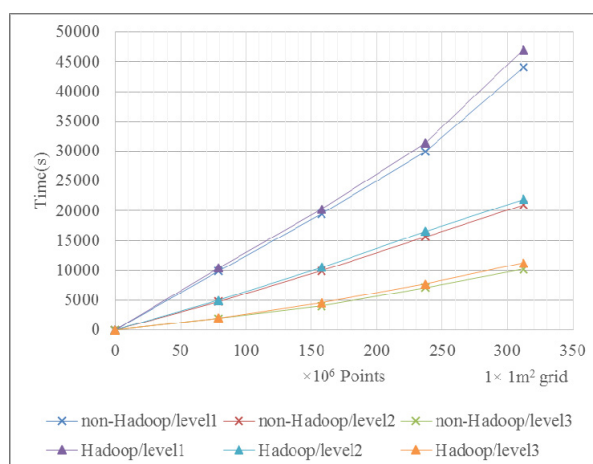
Figure 5(a).Hadoop and non-Hadoop approach
