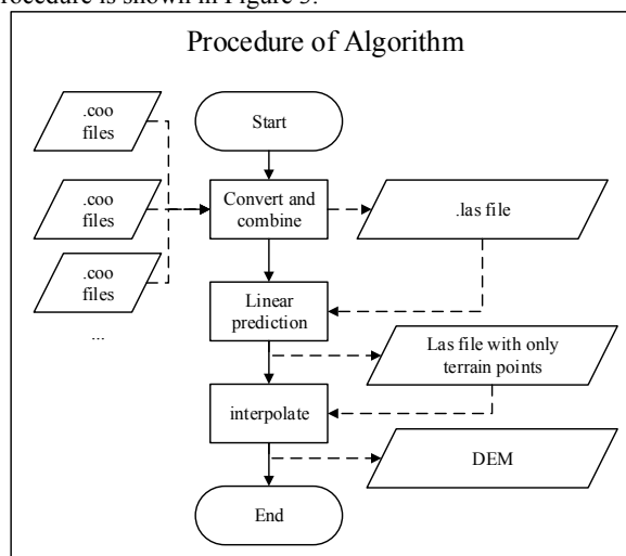
Figure 3. Procedure of Algorithm
