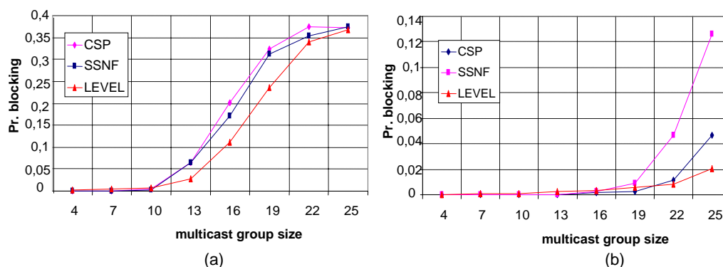
Figure 3: Blocking probability vs. multicast group size with (a) self-sharing and (b) self- and cross-sharing
