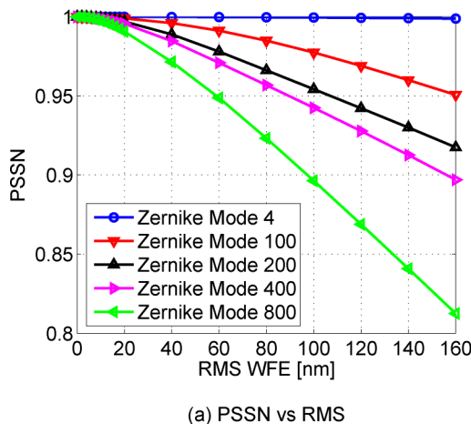
Fig. 5. (Color online) Numerically calculated PSSN for Zernike 4, 100, 200, 400, and 800 modes with respect to the RMS WFE: (a) PSSN plot in linear scale and (b) 1-PSSN plot in a log-log scale.
