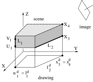
Figure 2: Relation between scene, image and drawing. Vertical line L_1 , passing through point U_1 , maps to l_1^d = u_1^d . Horizontal line L_2 has the same vanishing point as its projection l_2^d .
