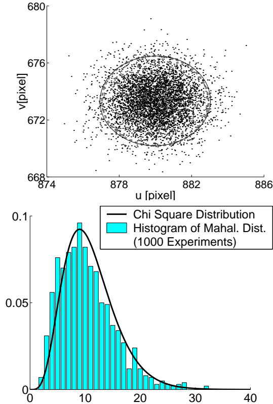
Figure 3: Top: Back-projection of a 3D point using estimated projection matrices. The projection is estimated based on randomly perturbed observations in the image and in the drawing. 5000 samples are taken to obtain the empirical 90% confidence region (solid), which is very close to the predicted one (dashed) from (5). Bottom: The Mahalanobis distance of the estimated projection matrix and the true projection matrix is \chi_{11}^2 distributed. The histogram represents the distribution obtained by 1000 experiments on perturbed data. The curve indicates the true \chi_{11}^2 distribution. The mean Mahalanobis distance is 10.87, compared to 11, which is statistically not different.
