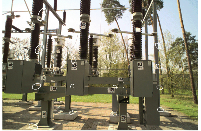
Figure 4: Uncertainty of projected 3D points. The ellipses show the covariances of 3D points on the ground, and points above of each in heights of 100, 200, and 300 pixels. The ellipses are plotted magnified by a factor of 10 for better visibility. In this case, the ground plane is not located on the actual ground, but at the top edge of the concrete foundations.
