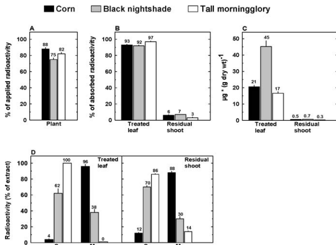
Figure 3. Foliar uptake (A), translocation (B, C), and metabolism (D) of [ 14 C]saflufenacil in light-grown plants of corn, black nightshade, and tall morningglory. Plants at the third-leaf stage were foliar treated with EC-formulated [ 14 C]saflufenacil with the addition of Dash HC ® at equivalents to field rates of 60 g ai ha -1 and 1 L ha -1 , respectively. After treatment for 16 h, radioactivity taken up in the leaf tissue and translocated beyond was determined by combustion analysis. Data are averages of 10 replicate plants. For study of metabolism (D), radioactivity was extracted from the plant material and analysed by high performance liquid chromatography (HPLC) radiocounting. Radioactivity in % of total extract found in the peaks of saflufenacil (Sa) and totalled metabolites (Me) was shown. Data are averages from three replicate extractions of three plants, respectively. Vertical bars represent standard error (SE) of the mean.
