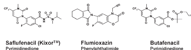
Figure 1. Structures of protoporphyrinogen IX oxidase (PPO)-inhibiting pyrimidinediones saflufenacil (Kixor™) and butafenacil, and phenylphthalimide flumioxazin.
