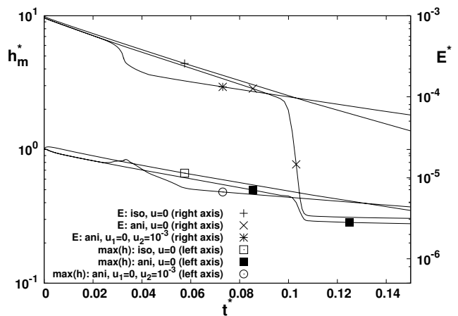
FIG. 2: Log plots for nondimensional maximum height, h_m^*(t) = h_m(t)/h_0 (left axis), and nondimensional surface energy, E^*(t) = E(t)\lambda_x^2/(h_0^3 g_3 \lambda_y) (right axis), vs nondimensional time t^* = tk_B T \lambda_1^5 / (h_0 D_s C_s g_3 \Omega^2) , for scalar (iso) and tensor (ani) cases without and with electric field (drift velocity \mathbf{v} \neq 0 in Eq. (5)); g_1 = 0 , q = 10^4 , h(x, y, 0) = h_0 \cos(k_1 x) \cos(k_2 y) , k_2/k_1 = \lambda_1/\lambda_2 = 11/24 , \mathbf{u} = (0, u_2) = \lambda_1 \mathbf{v}/D_s and \delta_1 = 10^{-5} . The presence of electric field causes an earlier transition (see Figs. 3 and 4).
