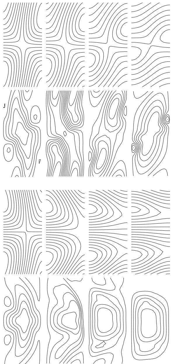
FIG. 4: Snapshots of height level sets (first and third rows) and adatom vector flux streamlines, i.e., curves tangential to flux (second and fourth rows) during transition, shown in the box [0, \lambda_1/2] \times [0, \lambda_2/2] . Streamlines are not normal to level sets, thereby reflecting the tensor nature of mobility, and exhibit a tendency to align with the y -axis for increasing time (from left to right). Upper two rows: \mathbf{E}_e = 0 . Lower two rows: \mathbf{E}_e \neq 0 in y -direction with |\mathbf{u}| = \lambda_1 |\mathbf{v}|/D_s = 10^{-3} (see Eq. (5)). Parameter values: g_1 = 0 , q = 10^4 , h(x, y, 0) = h_0 \cos(k_1 x) \cos(k_2 y) , k_2/k_1 = 11/24 . The time scale for \mathbf{E}_e \neq 0 is shorter than for \mathbf{E}_e = 0 (see also Fig. 2).
