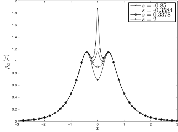
(a) The charge density \rho_Q(x) .
