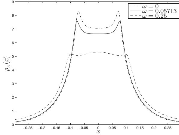
(a) The energy density \rho_E(x) .
