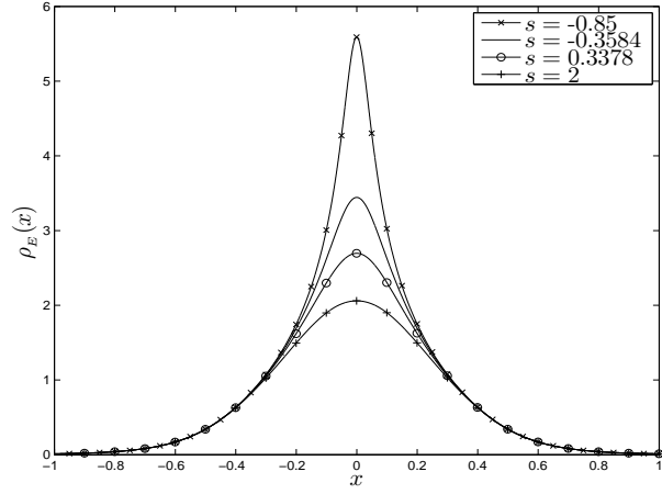
(b) The energy density \rho_E(x) .
