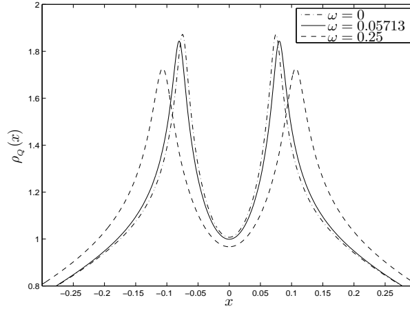
(b) The charge density \rho_Q(x) .
