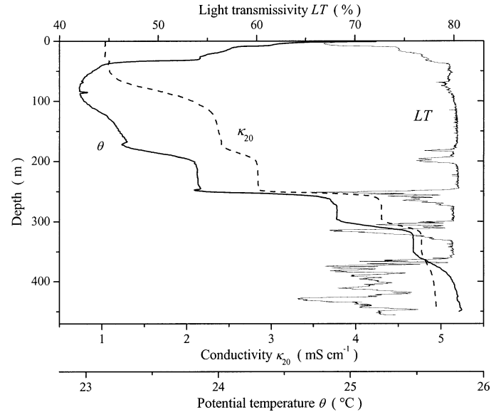
Fig. 2. Profiles of potential temperature, electrical conductivity corrected to 20°C, and light transmissivity, LT , from a CTD cast in the center of Lake Kivu northern basin (CTD Sta. 1 in Fig. 1).
