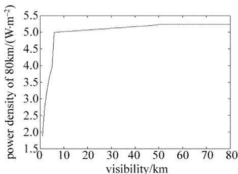
Fig. 2 Relation between power density and visibility
