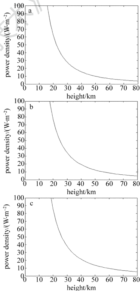
Fig. 3 The increase in power density with height from 0km to 80km at different visibility
