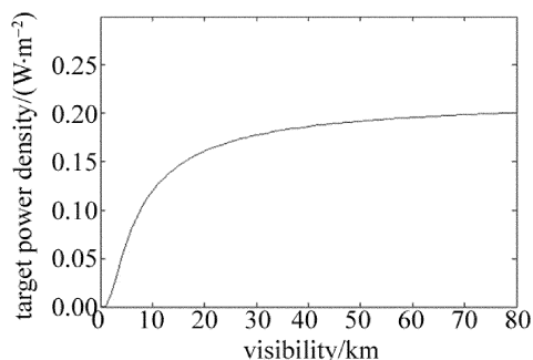
Fig. 4 The target power density curves at different visibilities
