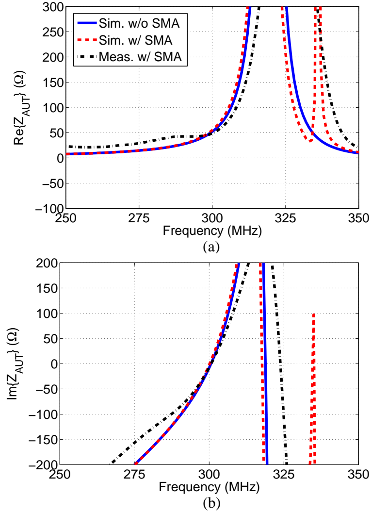
Figure 5.4. Comparison of the simulated and measured Z_{\text{AUT}} with direct excitation with semi-rigid coaxial cable in a reduced vertical axis scale. (a) \text{Re}\{Z_{\text{AUT}}\} . (b) \text{Im}\{Z_{\text{AUT}}\} .
