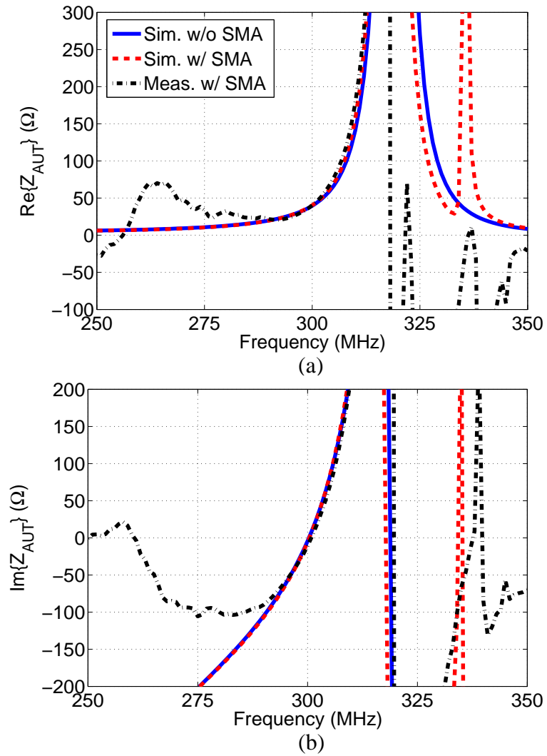
Figure 4.18. Comparison of the simulated and measured Z_{\text{AUT}} with d = 50 cm in a reduced vertical axis scale. (a) \text{Re}\{Z_{\text{AUT}}\} . (b) \text{Im}\{Z_{\text{AUT}}\} .
