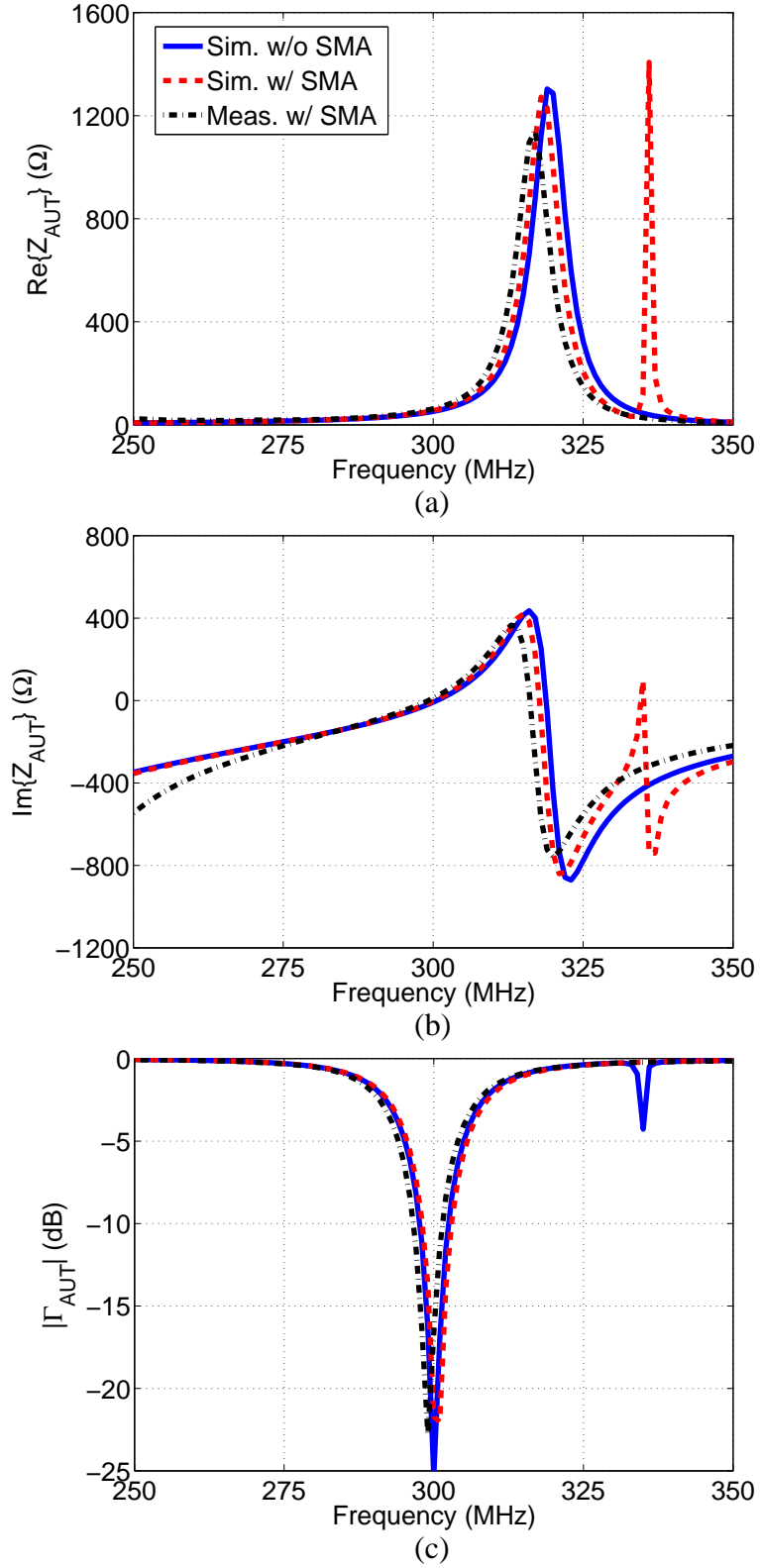
Figure 5.9. Comparison of the simulated and measured Z_{\text{AUT}} with direct excitation with semi-rigid coaxial cable and a two-wire line balun. (a) \text{Re}\{Z_{\text{AUT}}\} . (b) \text{Im}\{Z_{\text{AUT}}\} . (c) |\Gamma_{\text{AUT}}| .
