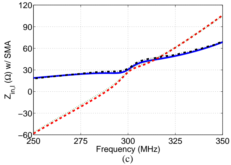
Figure 4.15. Comparison of the simulated and measured Z_{in} at port 1 with d = 25 cm. (a) The short standard case. (b) The open standard case. (c) The termination standard case. These impedances are referenced at the base of the monopole.
