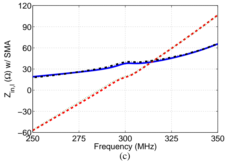
Figure 4.19. Comparison of the simulated and measured Z_{in} at port 1 with d = 50 cm. (a) The short standard case. (b) The open standard case. (c) The termination standard case. These impedances are referenced at the base of the monopole.
