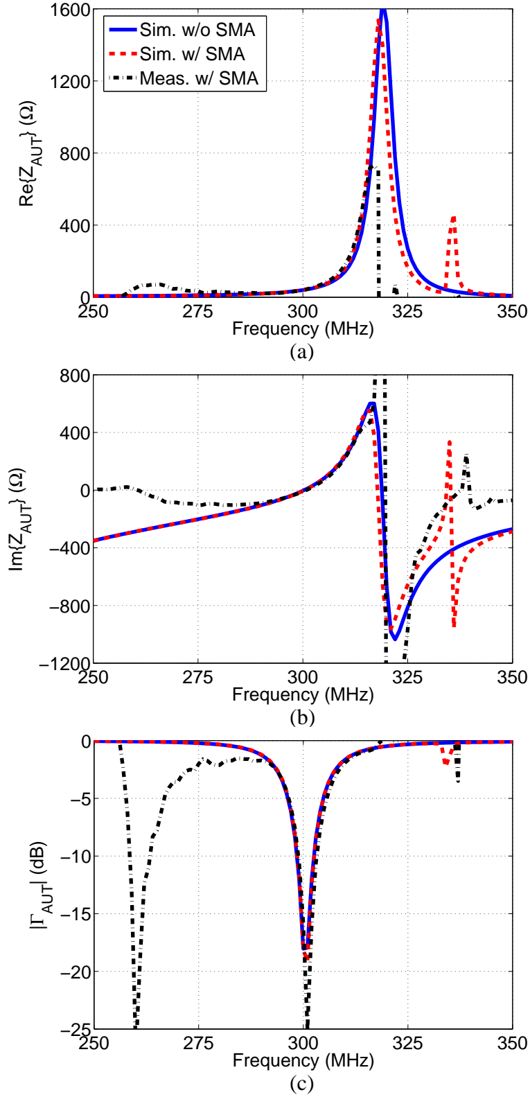
Figure 4.17. Comparison of the simulated and measured Z_{\text{AUT}} with d = 50 cm. (a) \text{Re}\{Z_{\text{AUT}}\} . (b) \text{Im}\{Z_{\text{AUT}}\} . (c) |\Gamma_{\text{AUT}}| . The impedances are referenced at the two-wire port of the connector.
