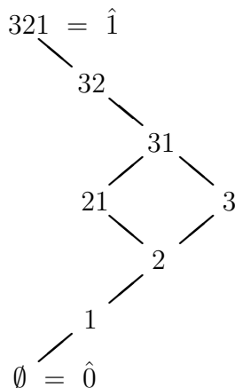
FIGURE 2. The Bruhat order for OG(3) .
