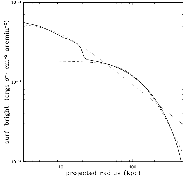
Fig. 3. Predicted bolometric surface brightness profile of the cluster displayed in Fig.1. The thick solid line is the resulting profile after the bubbles have been placed in the cluster. The dotted line is the best-fit isothermal \beta model, while the dashed line is the best-fit isothermal \beta model excluding the central 30 kpc. The sharp kink at \approx 20 kpc is an artifact of the simplistic geometry we have assumed for the bubbles. A more realistic geometry would result in a smoother surface brightness profile.
