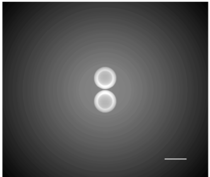
Fig. 1. Bolometric surface brightness map of a typical model cluster. The surface brightness is displayed in logarithmic scale. The solid white line indicates a length of 20 \text{ kpc} .
