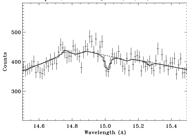
FIG. 2.— Fe xvii absorption line at 15.02\text{Å} in the Chandra MEG-LEG combined spectrum of 4U 1820–303, modeled with the absline model ( histogram ). The dip at 15.26\text{Å} indicates the expected amount of absorptions for the second most significant Fe xvii line (Table 1). The dotted line indicates the smooth continuum level around the line. The model has been convolved with the instrumental response, and the binsize is 12.5\text{mÅ} . The apparent bump on the blue-side of the line may be due to the imperfect calibration near the hot pixel. For the detail information of the co-added spectrum and the continuum fit, please refer to Paper I.
