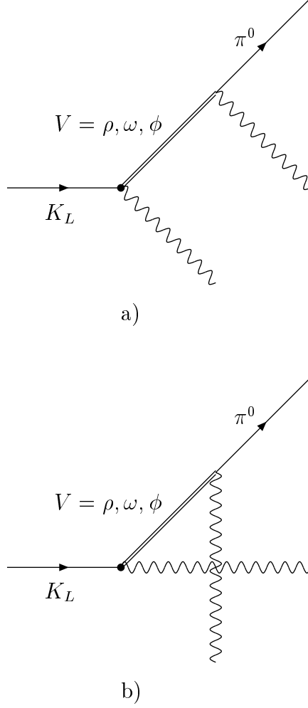
Figure 5: Vector meson exchange diagrams contributing to K_L \rightarrow \pi^0 \gamma e^+ e^- with unknown strength.
