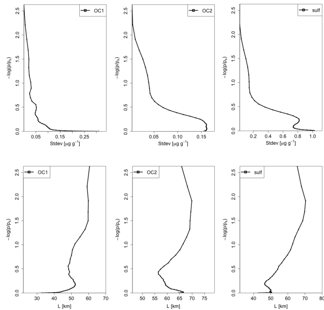
Figure 1. Vertical profiles of standard deviations (top) and horizontal correlation length scales (bottom) for OC 1 , OC 2 , and sulfate derived for a North American domain (see text for details). Tick mark values of -\log(p/p_s) on the ordinate approximately correspond to values of atmospheric pressure equal to 1000, 600, 370, 220, 135, and 80 hPa.
