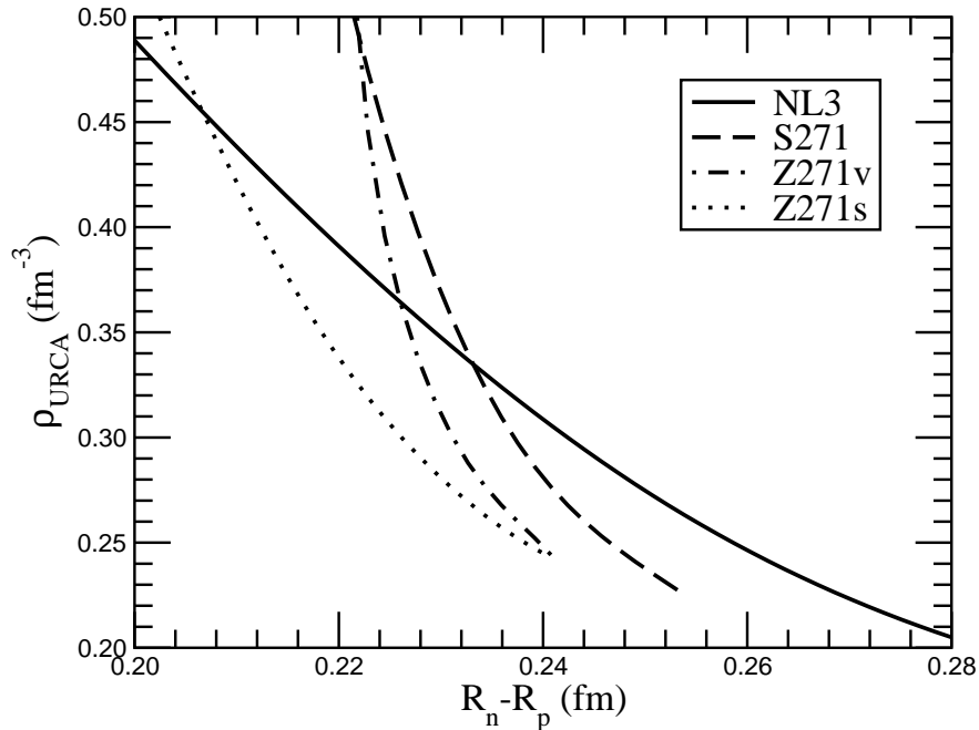
Figure 2.7: From Horowitz and Piekarewicz[22], the density direct Urca cooling occurs as a function of neutron skin thickness for various mean-field models.
