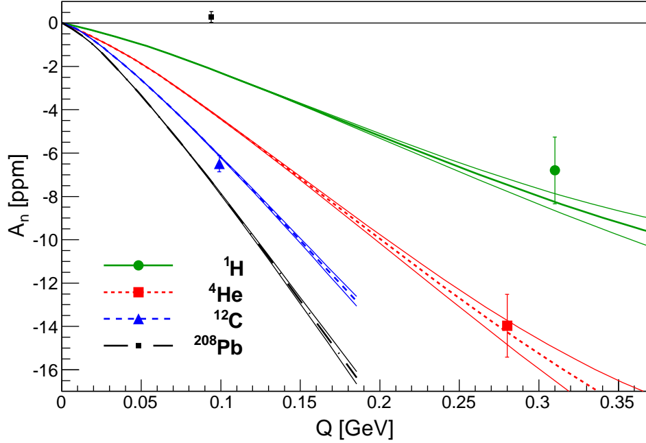
Figure 5.35: From Abrahamyan et. al.[46], the measured transverse asymmetries for ^1\text{H} , ^4\text{He} , ^{12}\text{C} and ^{208}\text{Pb} , shown with predictions. The ^1\text{H} , ^4\text{He} , and ^{12}\text{C} measured values agree with the model predictions for the transverse asymmetry, while the ^{208}\text{Pb} asymmetry does not.
