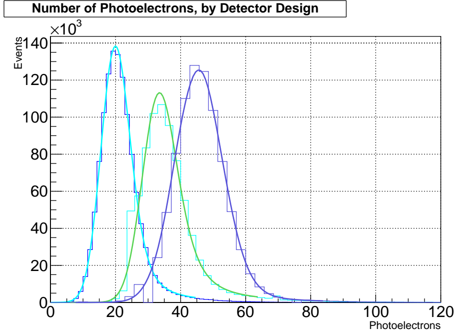
Figure 4.30: Fits for the PREX (light blue, 19 PE), flat design prototype (green, 32 PE) and angled prototype (purple, 44 PE) runs on the center of the quartz.
