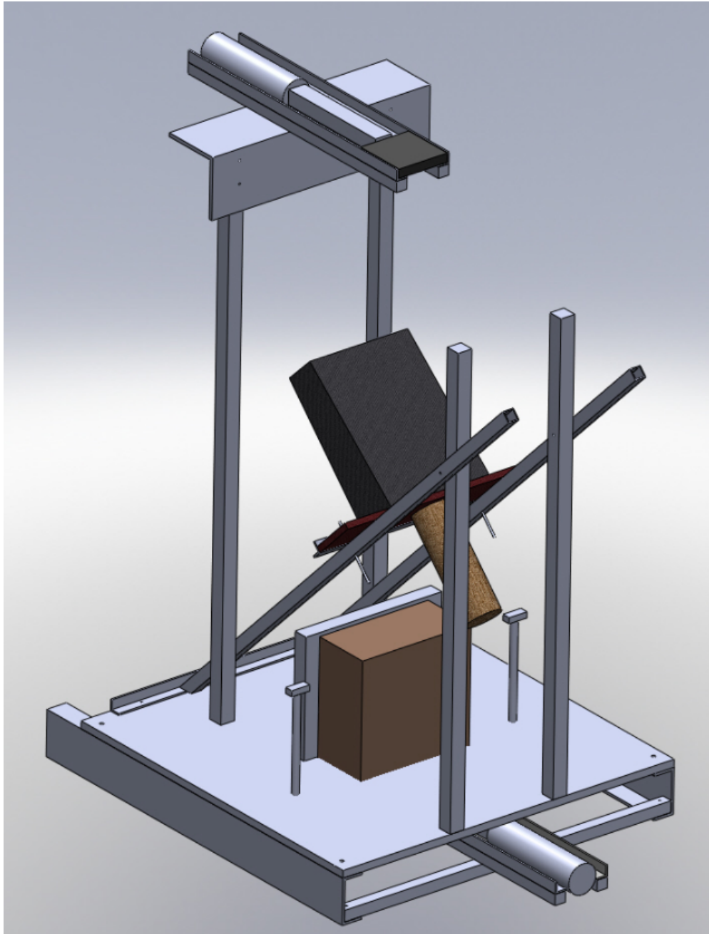
Figure 4.19: Stand design for the cosmic tests run at UMass-Amherst. Cosmic rays pass through the active region of the upper scintillator then through the quartz. The four 5 cm thick lead bricks, used to reject low energy rays, rest on a \frac{1}{2} " thick aluminum plate, which is suspended above the second scintillator used for the gate signal.
