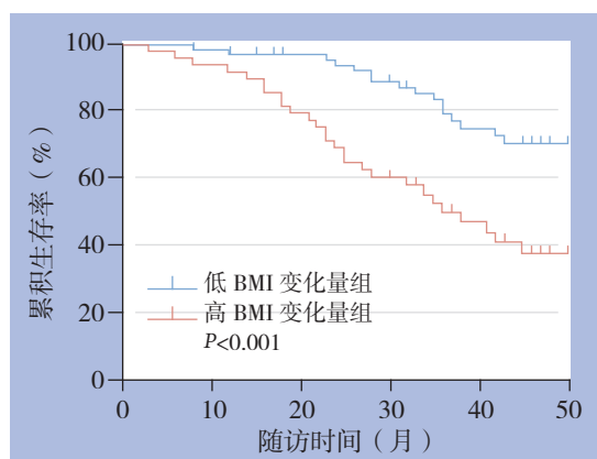
图 3 高 BMI 变化量组和低 BMI 变化量组患者生存曲线比较 Figure 3 Comparison of the survival curves between high BMI variation value and low BMI variation value
