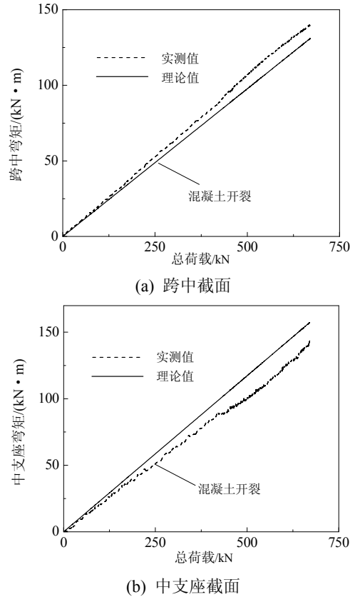
图 7 B6 梁的截面弯矩-荷载曲线 Fig.7 Load-flexural moment curve of specimen B6
