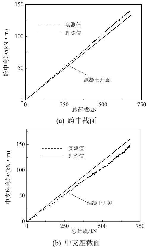
图 8 B7 梁的截面弯矩-荷载曲线 Fig.8 Load-flexural moment curve of specimen B7
