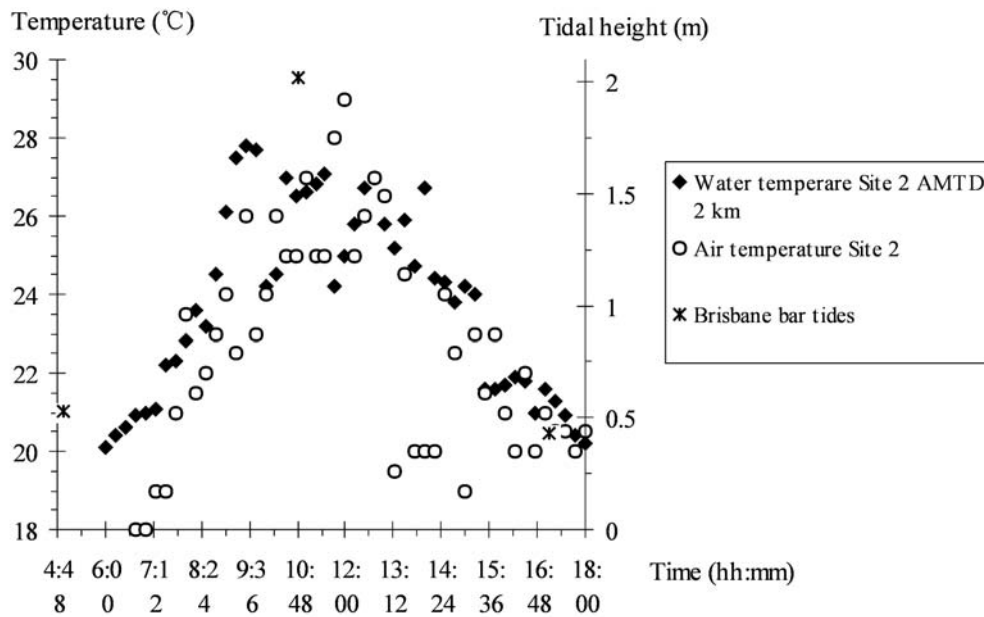
Fig. 3 Air and water temperatures at Site 2 (AMTD 2 km)- Comparison with Brisbane bar tides
