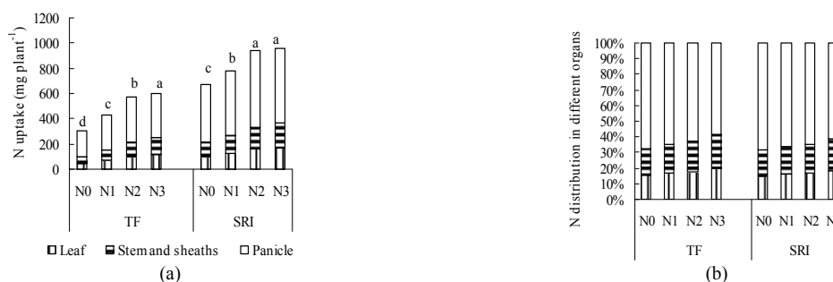
Figure 2. N uptake and distribution in stem and sheaths, leaf and panicle at maturing stage.
