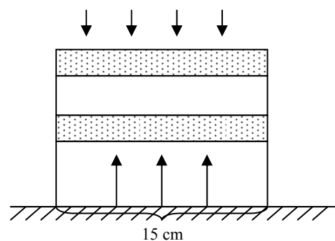
Figure 1. Design of instrument for collecting ammonia volatilization from the soil surface.
