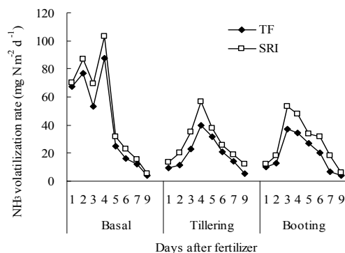
Figure 3. Average ammonia volatilization rates with four N rates after N fertilizer application at basal (May 19), tillering (June 29) and booting (July 29) stage under SRI and TF.
