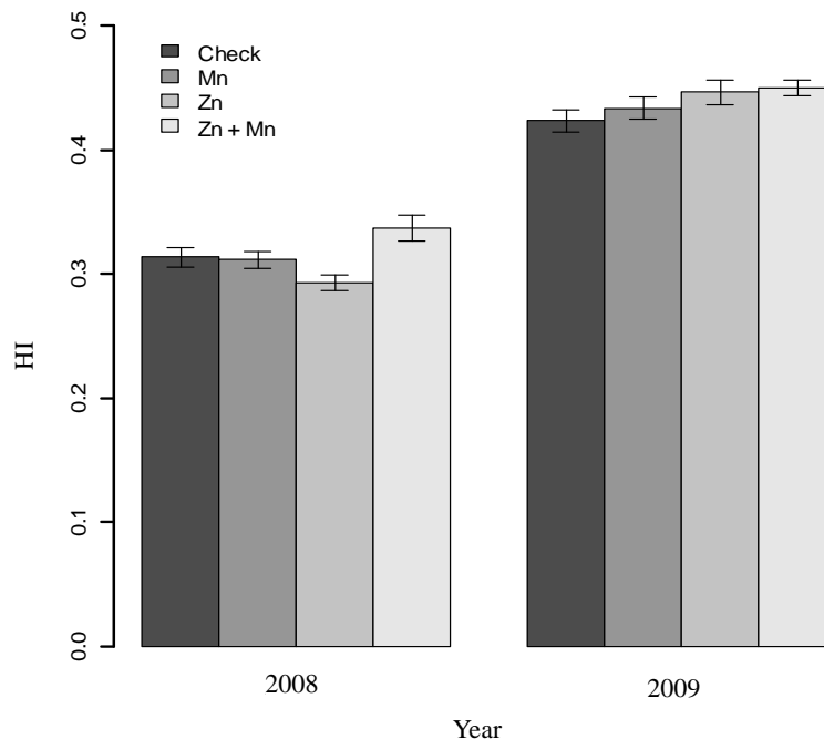
Figure 3. Effect of YR \times S interaction on harvest index in both seasons. P > F = 0.035 and 0.020 in 2008 and 2009, respectively. Error bars represent the standard error.
