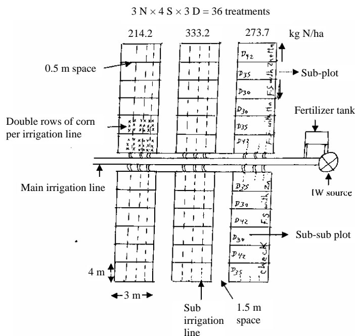
Figure 1. Layout of one replicate showing the study factors and plant distribution in the blocks.
