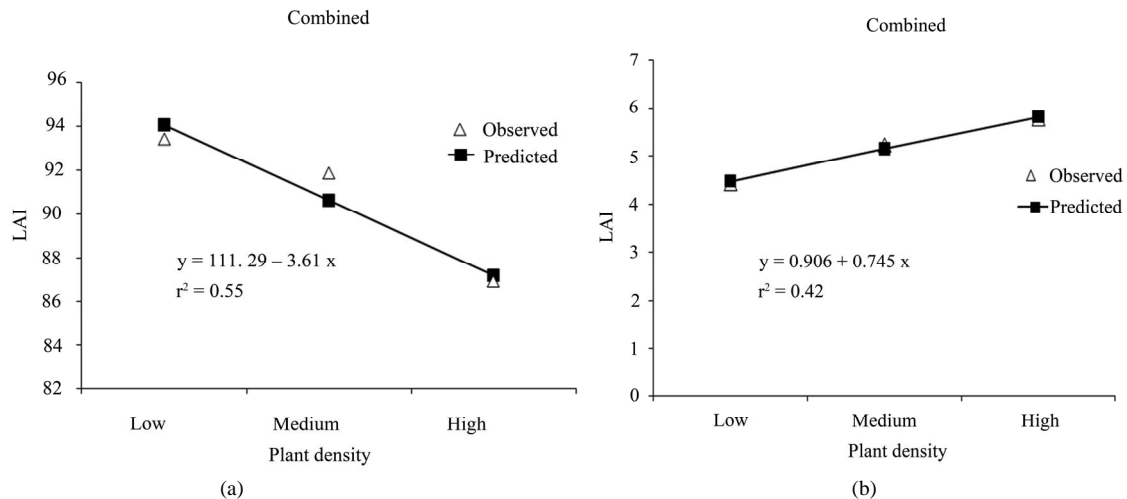
Figure 2. LA plant -1 (dm 2 ) (a) as a negative linear function in the pooled data and LAI (b) as a positive linear function in the pooled data.
