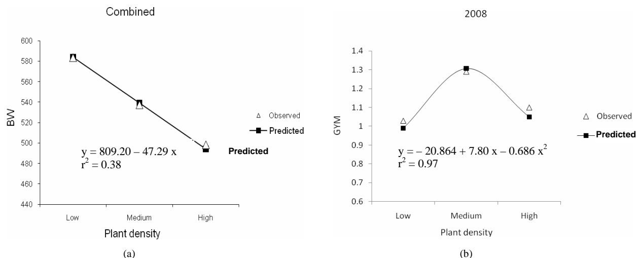
Figure 4. Plant weight ( \text{g}\cdot\text{plant}^{-1} ) (a) as a negative linear function of plant density in the pooled data and GYM ( \text{kg}\cdot\text{m}^{-2} ) (b) as a quadratic function of plant density in 2008.
