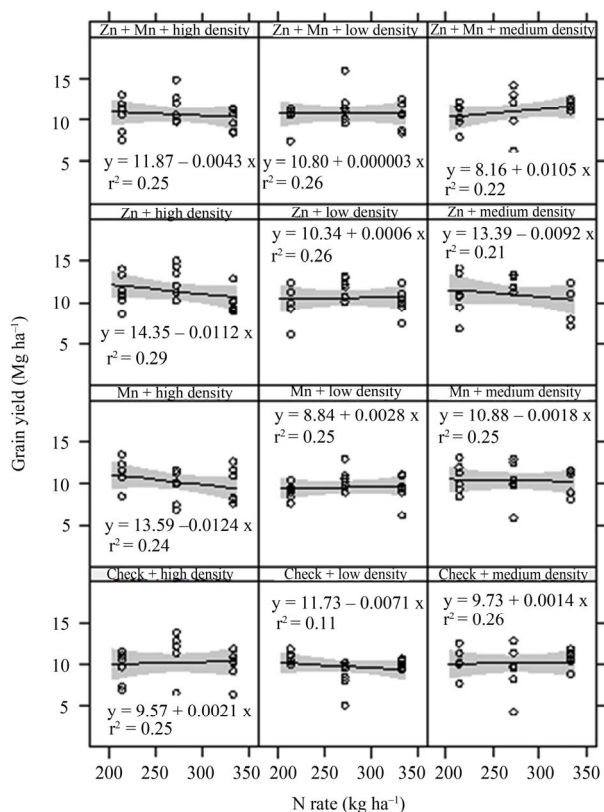
Figure 5. Effect of \text{N} \times \text{S} \times \text{D} interaction on grain yield ( \text{Mg}\cdot\text{ha}^{-1} ) over seasons. Shaded areas are 95% confidence intervals of the response curve.
