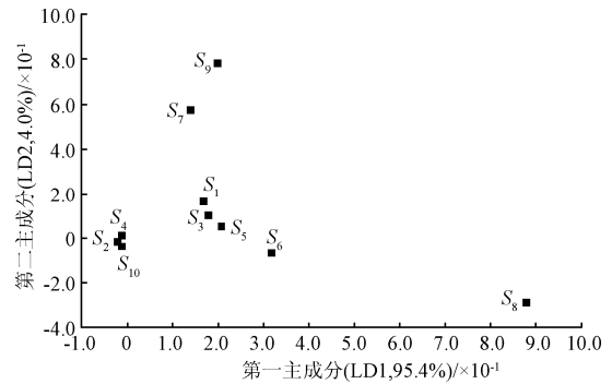
图 5 草莓接种处理 2 d 后响应信号的载荷分析 Fig.5 Loading analysis for response of strawberries after 2 days of inoculation
