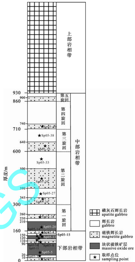
图 2 岩性剖面图及取样点 Fig. 2 Lithologic profile and sampling point
