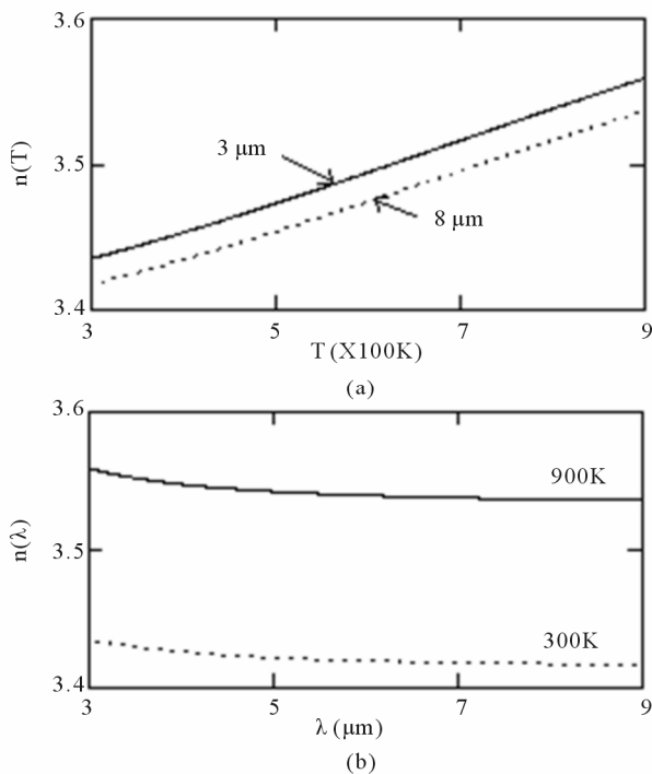
Figure 2. Variation of refractive index (a) with temperature at constant wavelength; (b) with wavelength at constant temperature.
