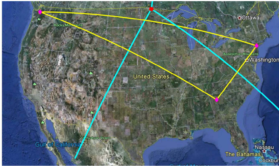
Figure 6. The spherical Voronoi Diagram for the 3 data centers, in Seattle, Atlanta, and New York. The arcs of the great circles connecting Seattle to Atlanta, Seattle to New York, and Atlanta to New York are shown by yellow lines. The cyan lines are the spherical bisectors between these cities. The cyan lines intersect at a point which is the vertex of the Voronoi Diagram.
