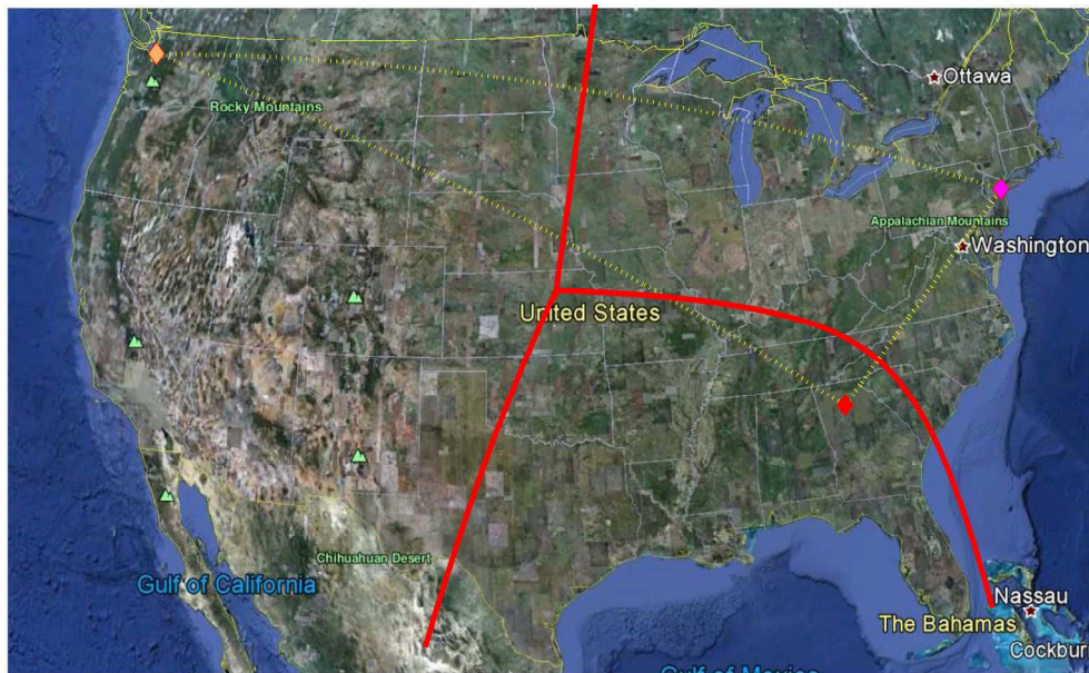
Figure 7. The solution to the constrained minimization problem with the 3 data centers, in Seattle, Atlanta, and New York. The solution is shown by a thick red line.
