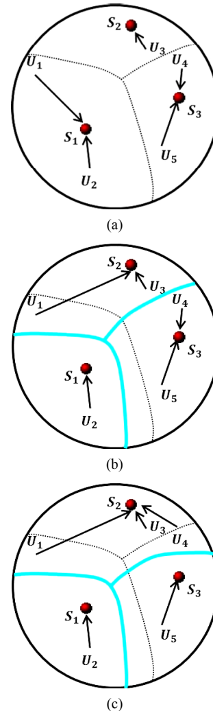
Figure 4. Three data centers. (a) No constraints; (b) One constraint; (c) Two constraints.
