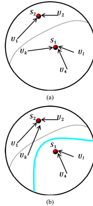
Figure 2. Two data centers with and without capacity constraints. (a) Without constraints; (b) With constraints.
