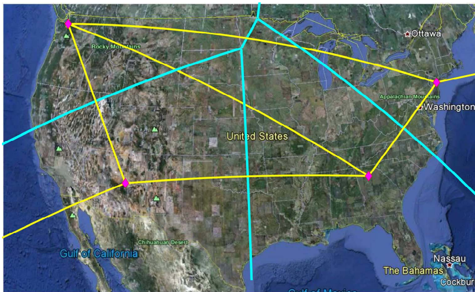
Figure 8. The Voronoi Diagram on the sphere for the 4 data centers, in Seattle, Atlanta, New York, and Phoenix. The arcs of the Delaunay Triangulation on the sphere for the 4 centers are shown by yellow lines. The cyan lines are the edges of the Voronoi Diagram.
