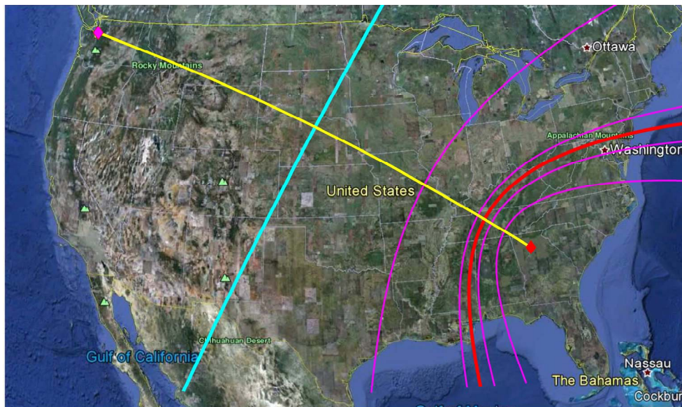
Figure 5. The solution to the constrained minimization problem with 2 data centers, in Seattle (the magenta diamond in the left upper corner) and Atlanta (the red diamond). The arc of the great circle connecting Seattle to Atlanta is shown by the yellow line. The cyan line is the spherical bisector between Seattle and Atlanta. The thin magenta lines show spherical hyperbolas which are the successive approximations to the hyperbolic Voronoi Diagram on the sphere, with the constraint of 80 million users in the Atlanta data center. The thick red line is the final approximation. The region inside the red line contains 79.4 million citizens, which are assigned to the Atlanta data center.
