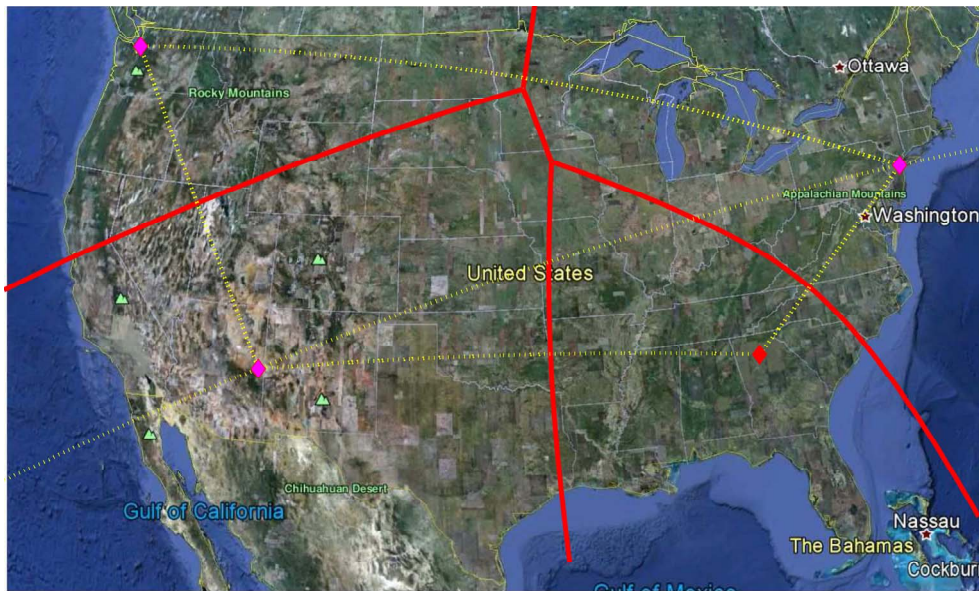
Figure 9. The solution to the constrained minimization problem with the 4 data centers, in Seattle, Atlanta, New York, and Phoenix. The solution is shown by a thick red line. Observe the bifurcation of the Voronoi Diagram from Figures 8-9.
