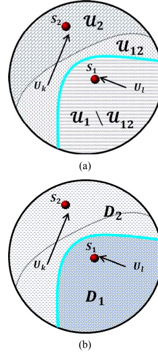
Figure 3. Solution for two data centers with capacity constraints. (a) Illustration for (13); (b) Regions D_1, D_2 .
