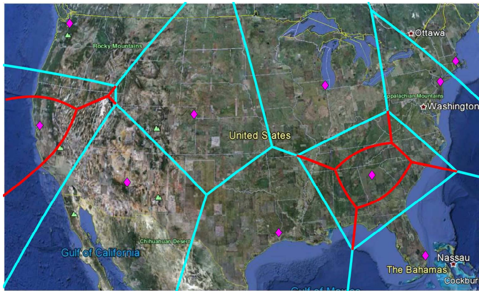
Figure 10. The solution to the constrained minimization problem with 10 data centers, Seattle, Atlanta, New York, Phoenix, San Francisco, Denver, Houston, Chicago, Boston, and Miami. The Voronoi Diagram on the sphere with these 10 points is shown by the cyan line. In this case, there are two constraints: in San Francisco the capacity is equal to 15 million users and in Atlanta it is 20 million. The constraints change the Voronoi Diagram locally near Atlanta and San Francisco to the hyperbolic diagram. The changes are shown in red.
