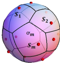
Figure 1. Voronoi diagram V on the sphere with the points \{S_m\} .
