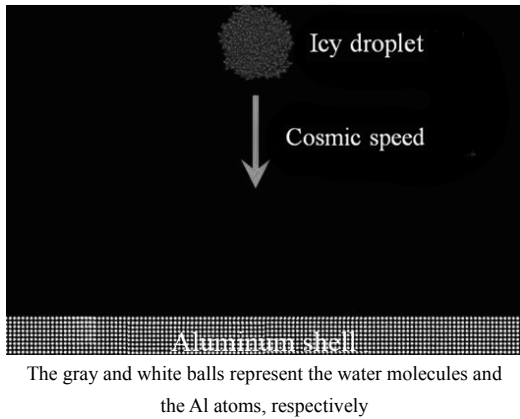
Fig. 1 Illustration of the MD simulation domain spacecraft Aluminum (Al) shell at nanoscale using molecular dynamics (MD) simulations accomplished in LAMMPS [6] . The simulation domain is illustrated in Fig.
