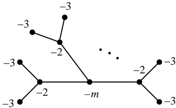
FIGURE 1. The plumbing diagram of the figure has at least n bad vertices (where n is the valency of the central (-m) -framed vertex) and it is either type-1 or rational (depending on the actual value of m ). Notice that all the (-2) -framed vertices are bad vertices (in the sense of Definition 2.1). On the other hand, for m sufficiently negative the graph is rational: let K be the vector which is the sum of all -3 -spheres, twice the -2 spheres, and once the central vertex. It follows that for any value of m the graph is of type-1.
