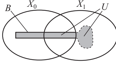
Figure 1: Proof of Lemma 3.4.
