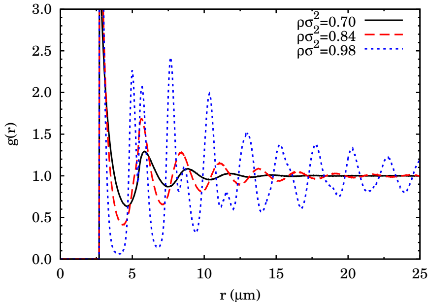
FIG. 3. (Color online) RDF for approximately one hemisphere of the colloidosome with D/\sigma = 23.8 and \sigma = 2.72 \mu\text{m} at a reduced temperature k_B T/\epsilon_{\text{PHS}} = 9.1 and various densities, calculated with a MC simulation of the PHS fluid.
